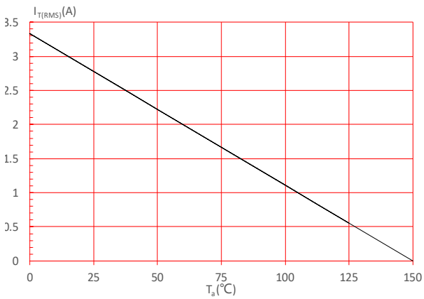
FIG.5: On-state characteristics
